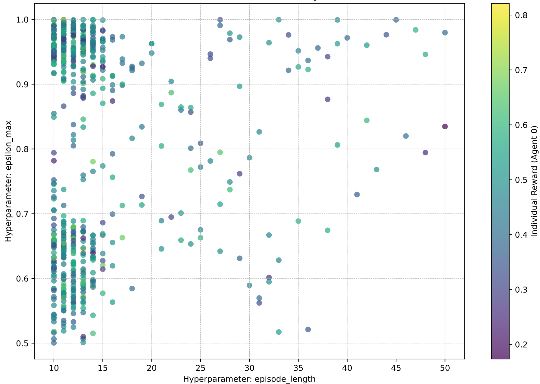
episode_length vs. epsilon_max (Color shows Individual Reward (Agent 0))
