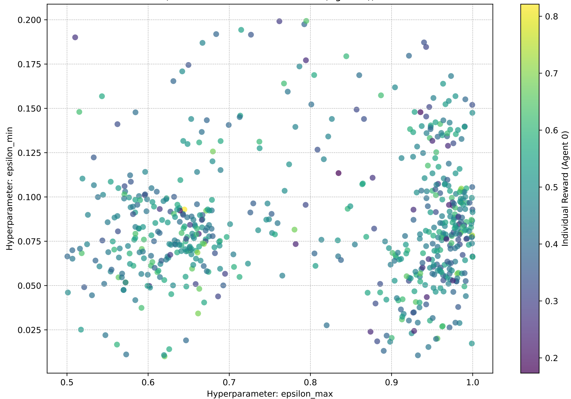
epsilon_max vs. epsilon_min (Color shows Individual Reward (Agent 0))
