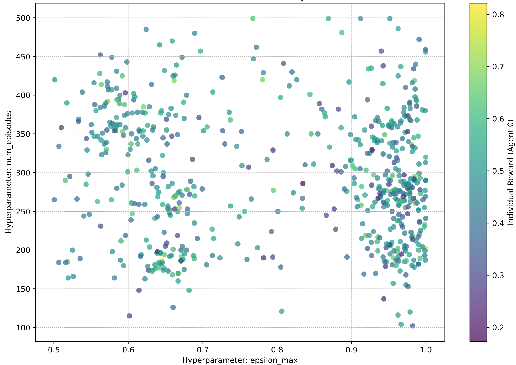
epsilon_max vs. num_episodes (Color shows Individual Reward (Agent 0))
