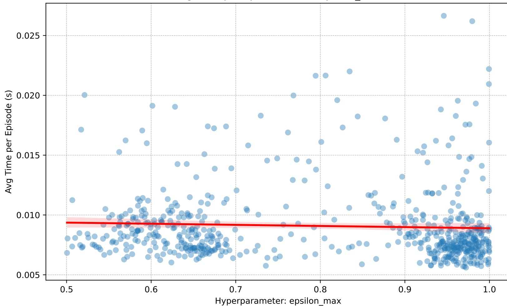
Avg Time per Episode (s) vs. epsilon_max
