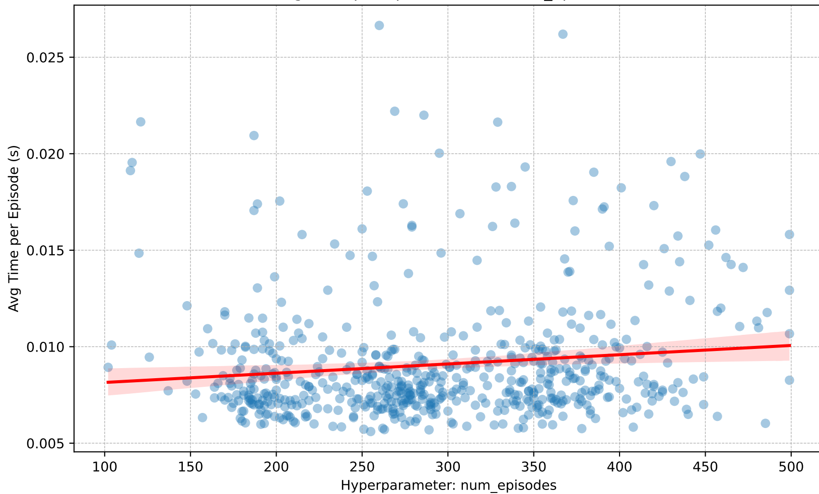
Avg Time per Episode (s) vs. num_episodes
