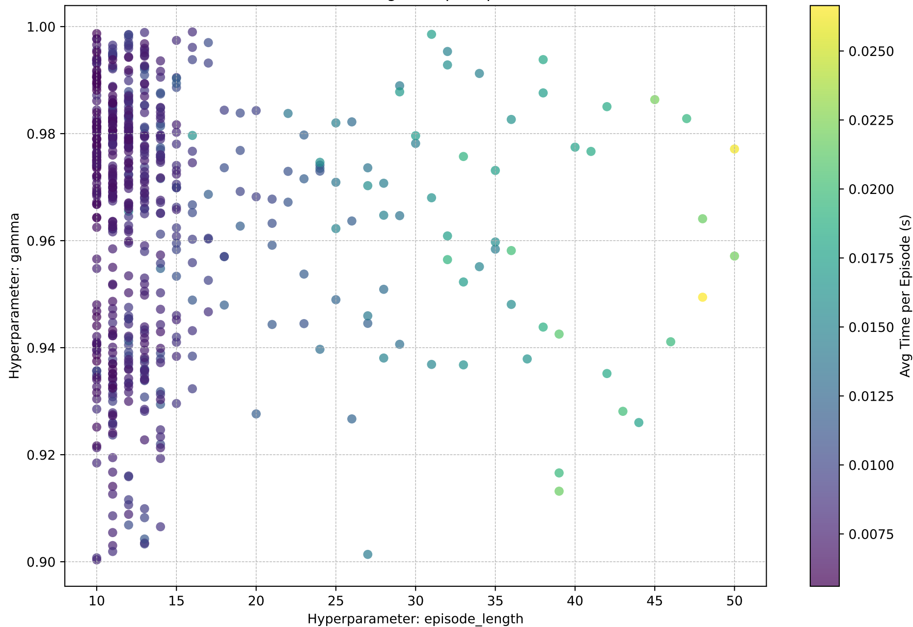
episode_length vs. gamma (Color shows Avg Time per Episode (s))
