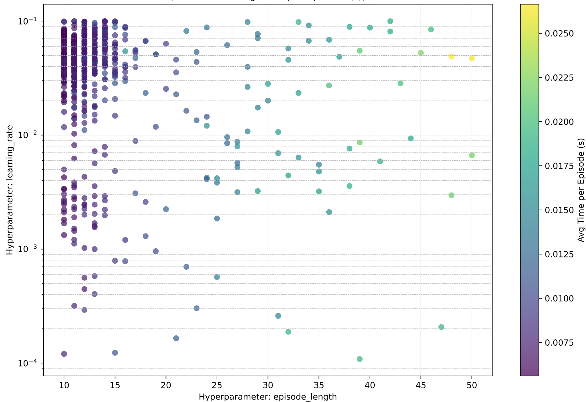
episode_length vs. learning_rate (Color shows Avg Time per Episode (s))
