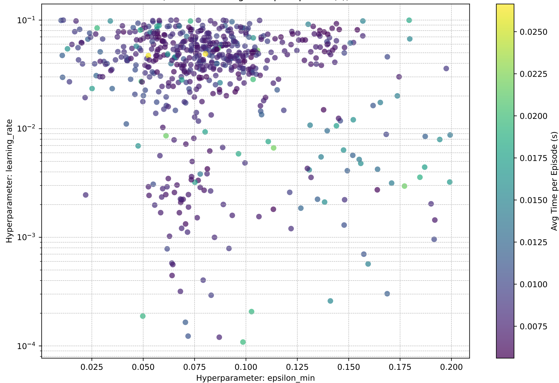
epsilon_min vs. learning_rate (Color shows Avg Time per Episode (s))
