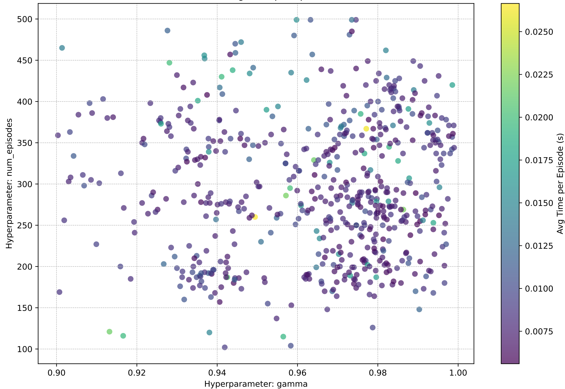
gamma vs. num_episodes (Color shows Avg Time per Episode (s))
