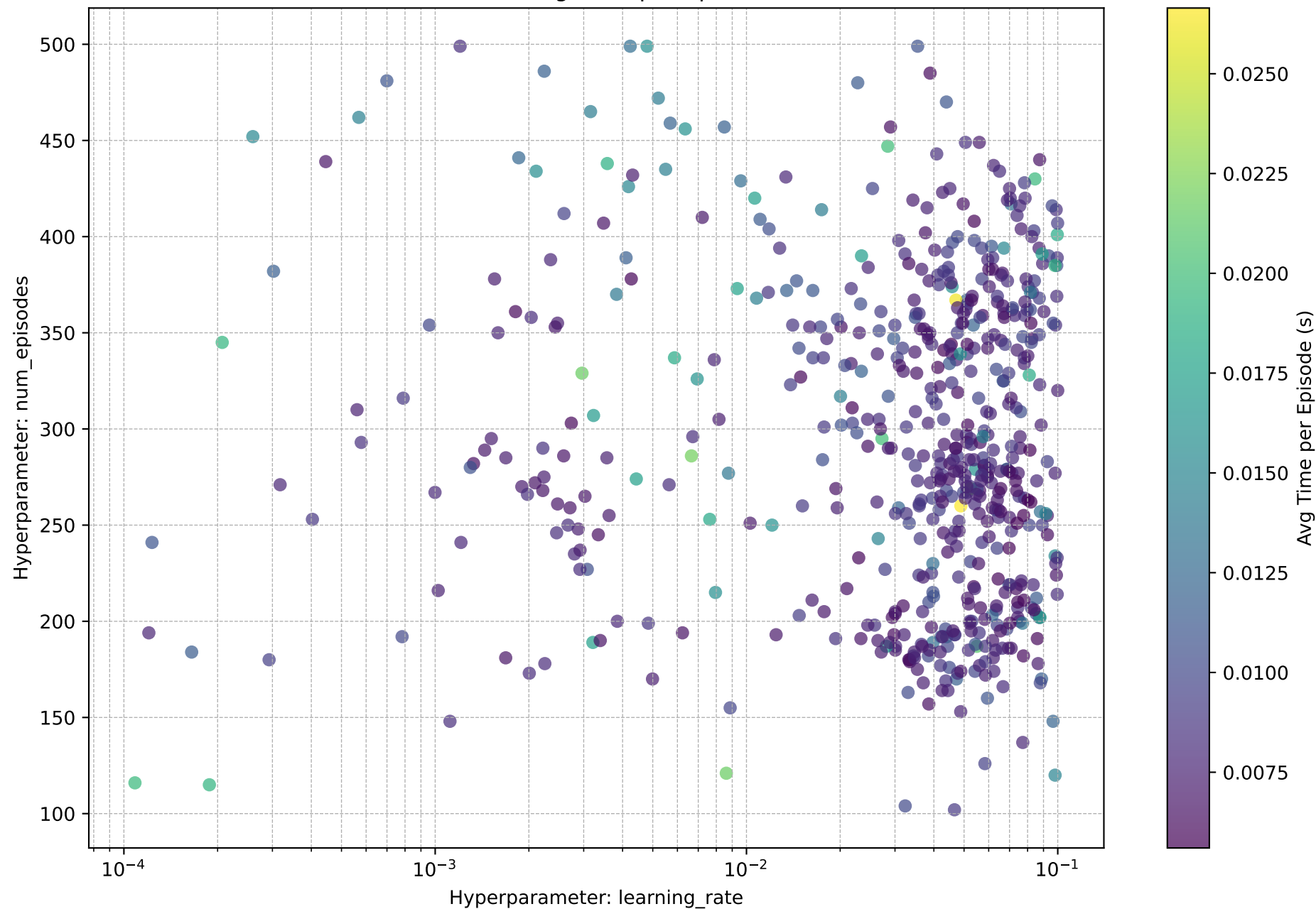
learning_rate vs. num_episodes (Color shows Avg Time per Episode (s))
