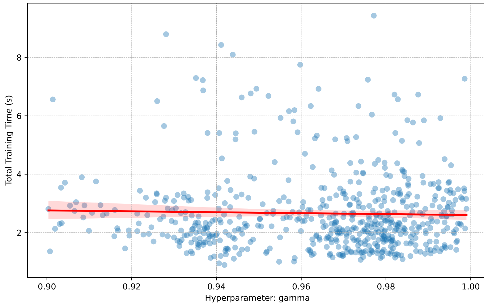
Total Training Time (s) vs. gamma
