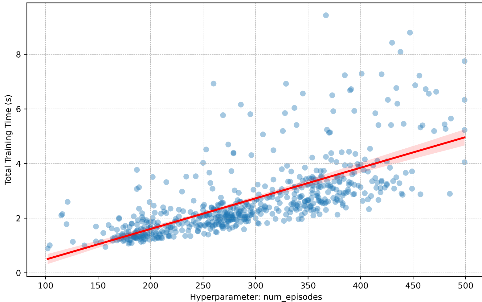
Total Training Time (s) vs. num_episodes
