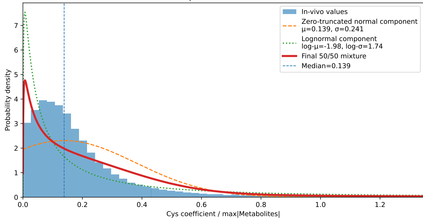
Cys coefficient ratio
