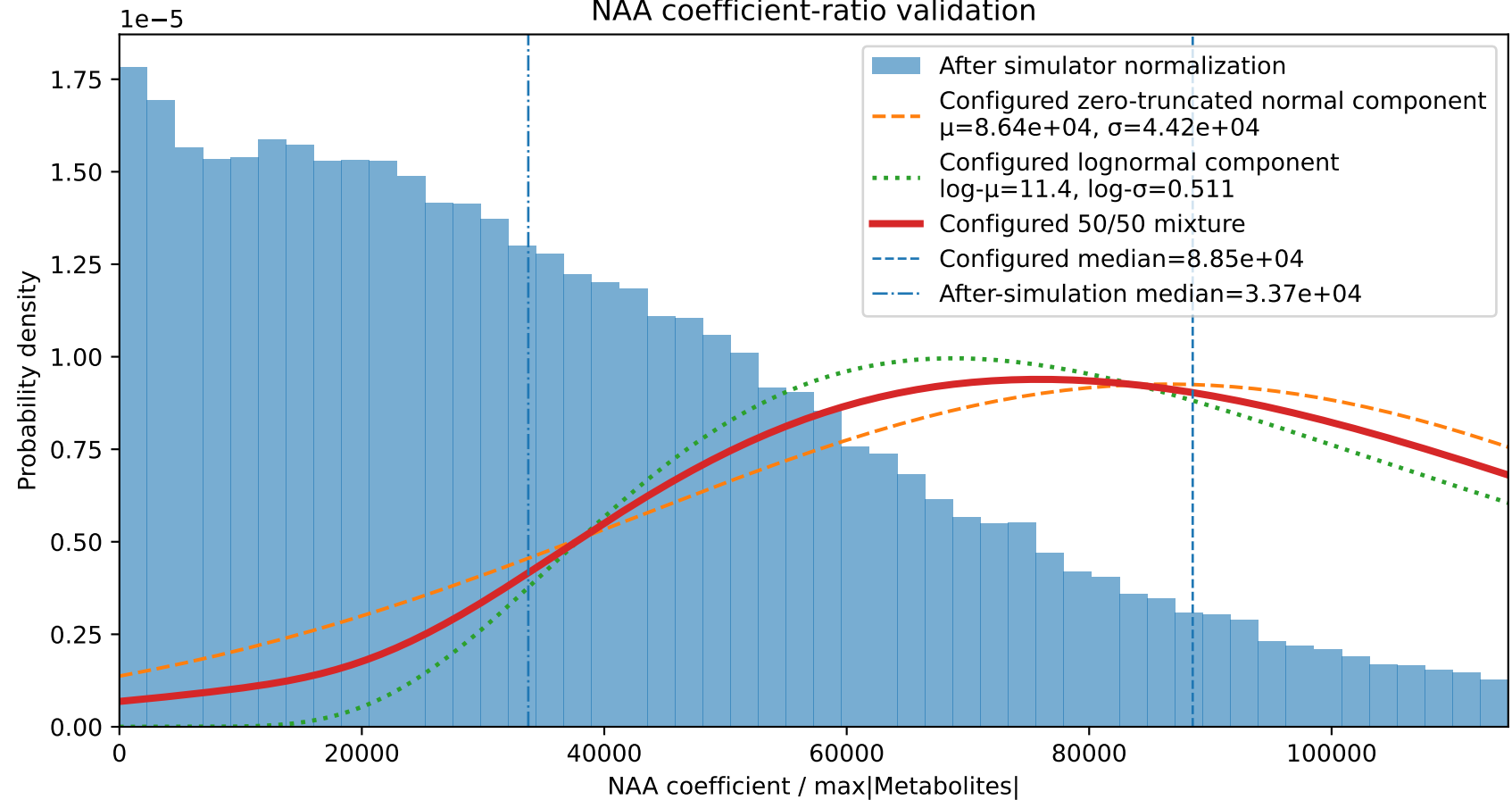
NAA coefficient-ratio validation
