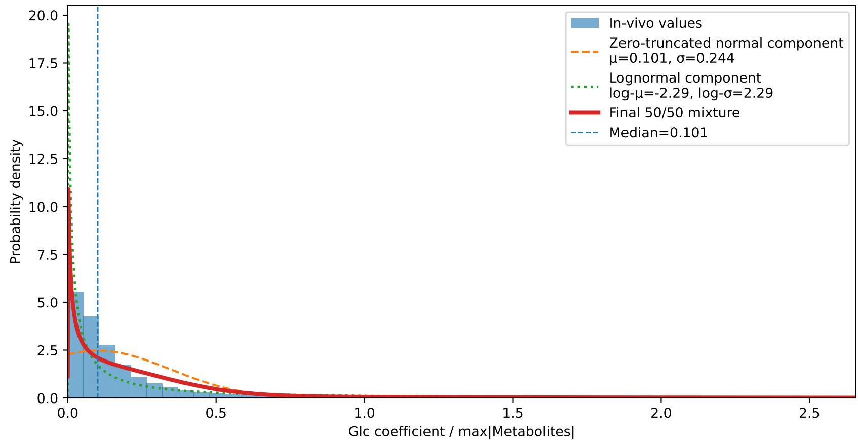
Glc coefficient ratio
