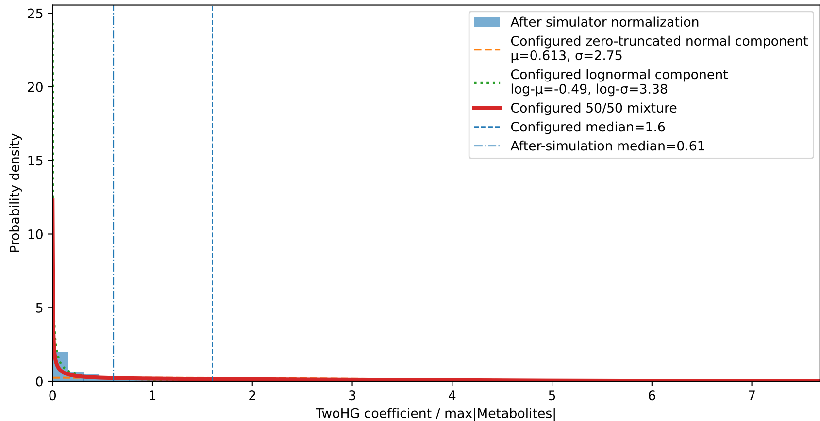
TwoHG coefficient-ratio validation
