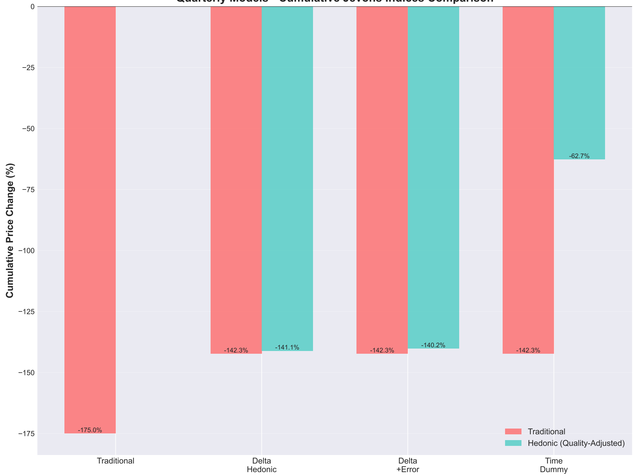
Quarterly Models - Cumulative Jevons Indices Comparison
