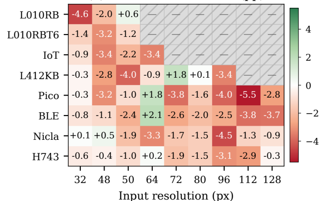
(b) Cancer: \Delta TFLite acc. (pp)
