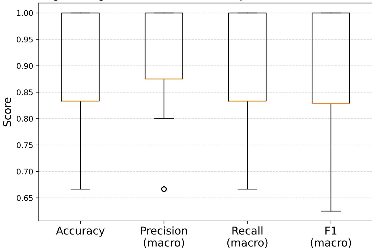
Logistic Regression 80/20 train-test splits (overall) — n=1000
