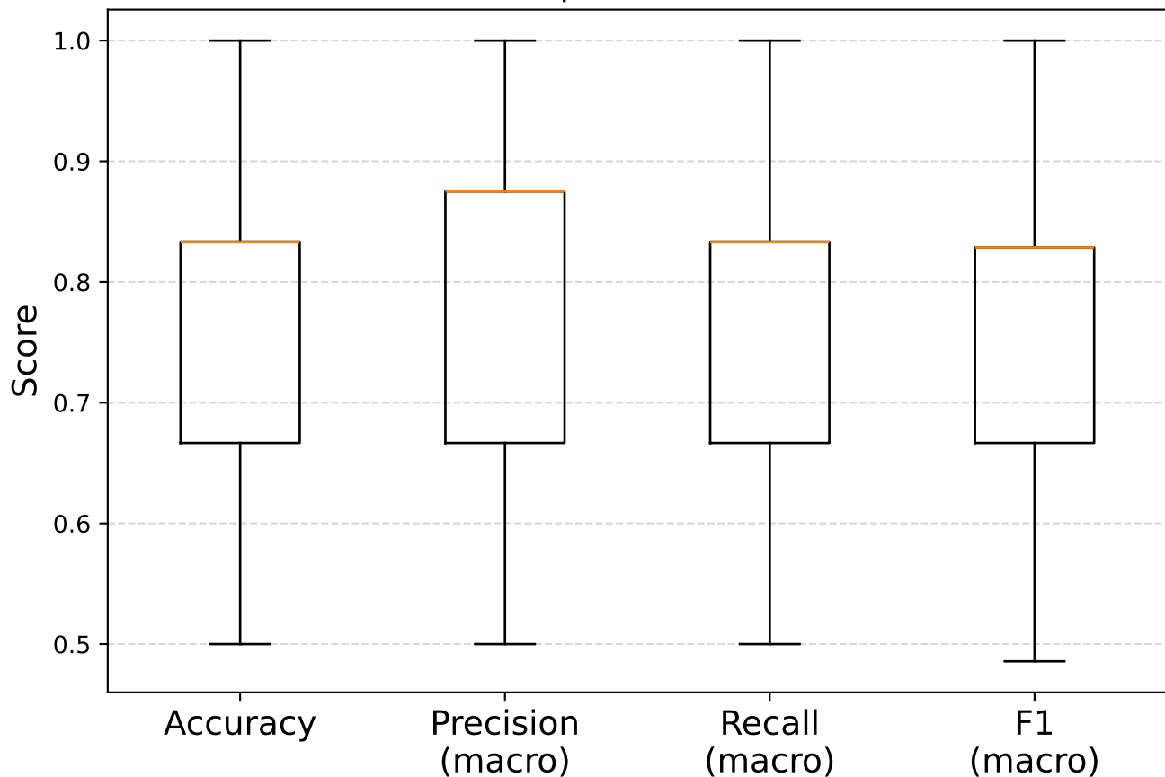
MLP on 80/20 splits (overall) — n=1000
