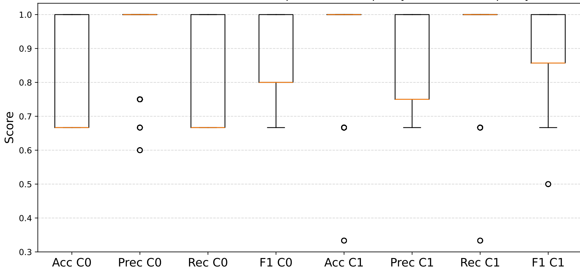
Per-class metrics 80/20 train-test splits (C0=Conspiracy, C1=Non-Conspiracy)
