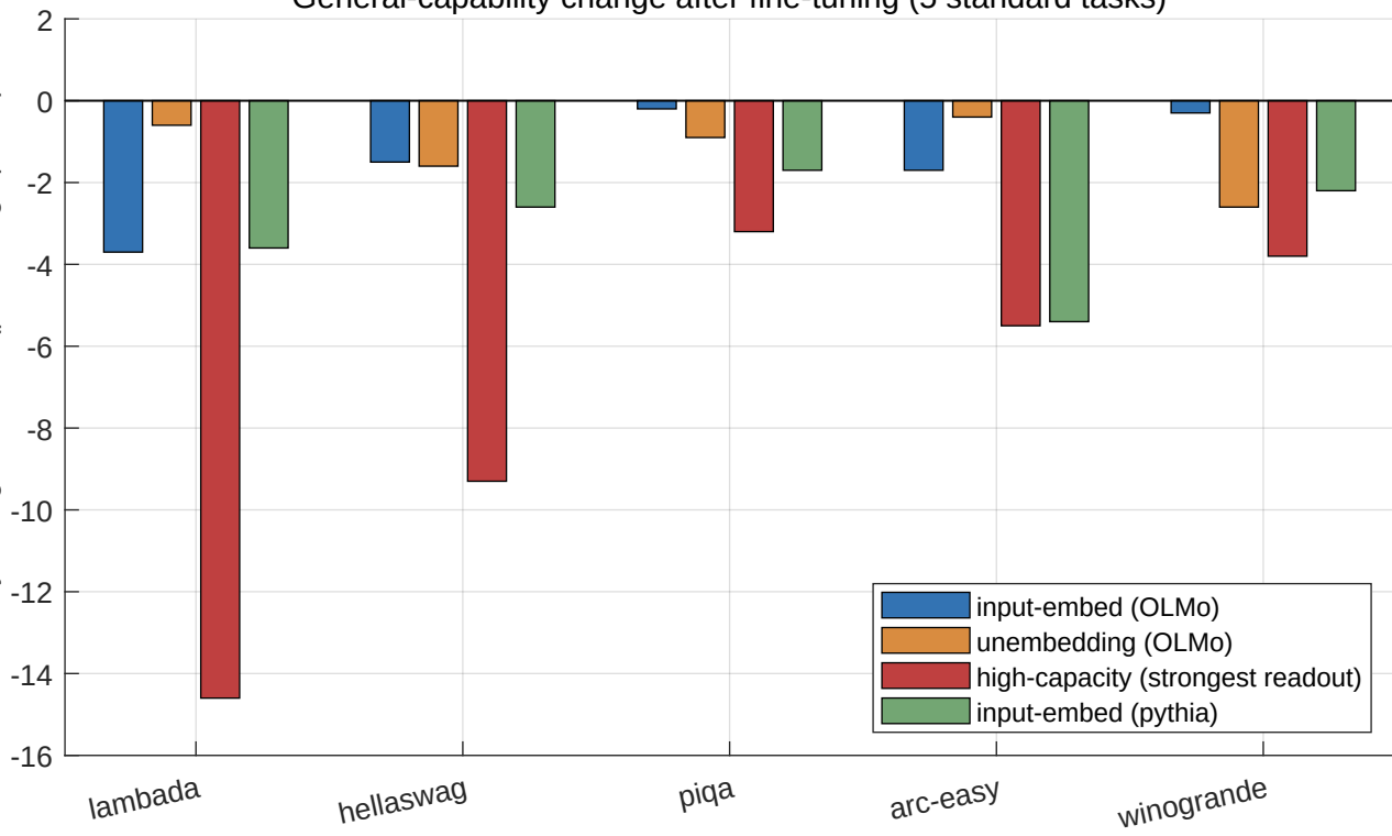
General-capability change after fine-tuning (5 standard tasks)
