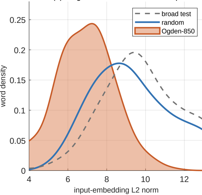
(a) magnitude: a small-norm clump
