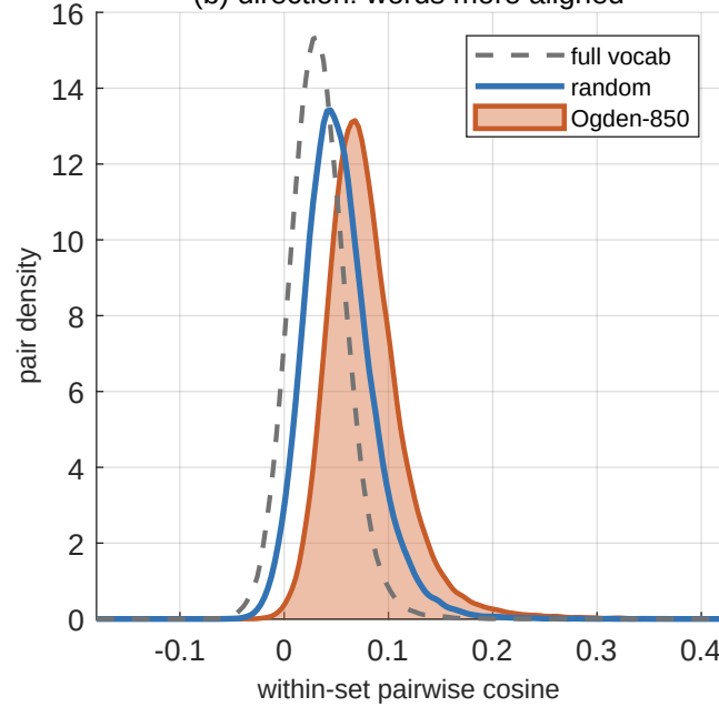
(b) direction: words more aligned
