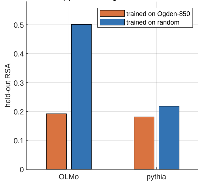
(c) -> weaker generalization
