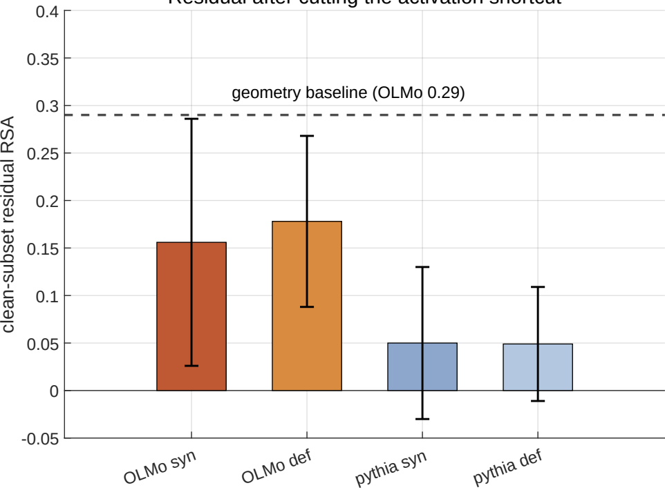
Residual after cutting the activation shortcut
