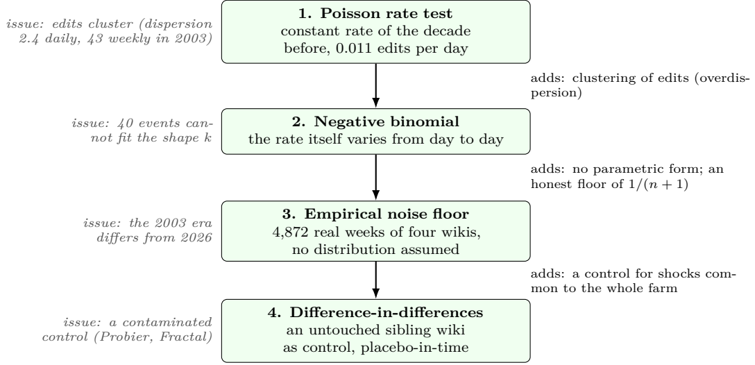
Figure 3: The four null models, what each adds to the previous one, and the issue that remains.
