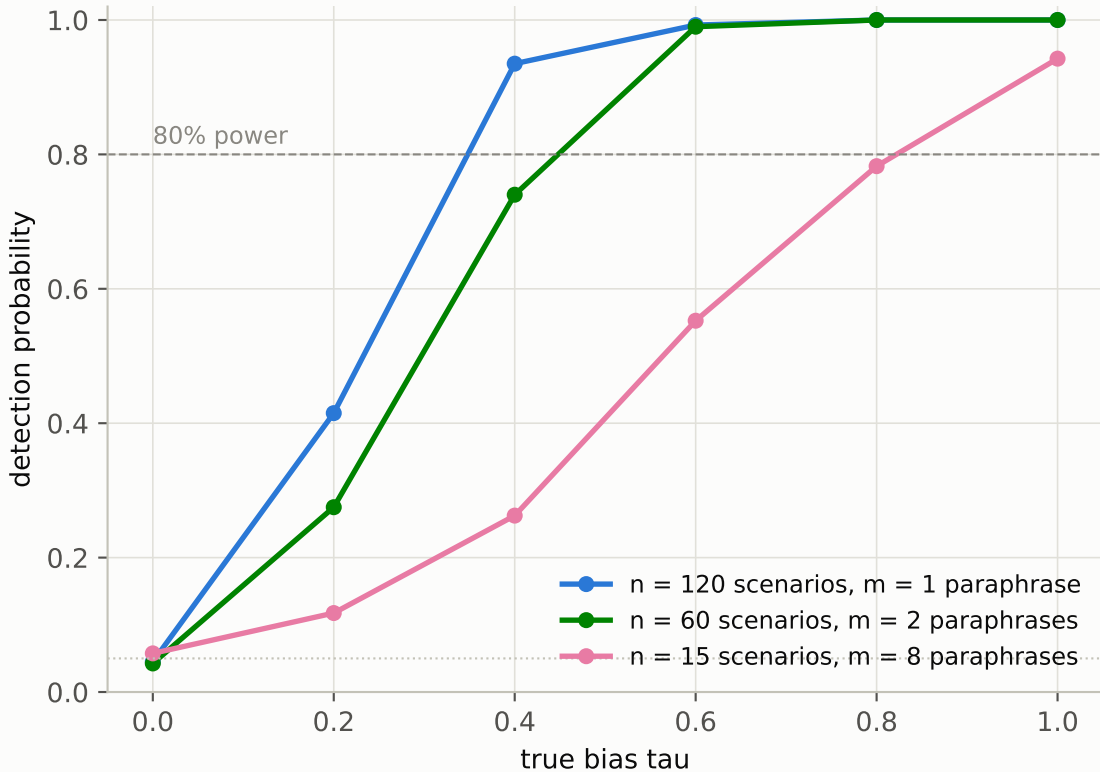
Same budget (120 queries per arm), different power
