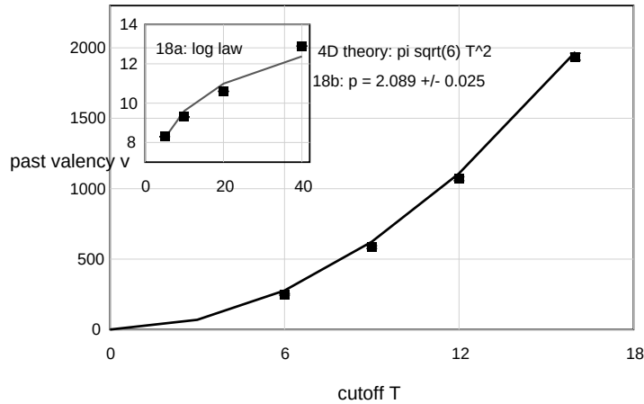
Figure 1: Past valency vs. cutoff: 2D logarithmic law and 4D area law. The 4D area-law curve is parameter-free ( \kappa_4 = \pi\sqrt{6} ); in 2D the slope 2 is derived and the O(1) offset is fitted.
