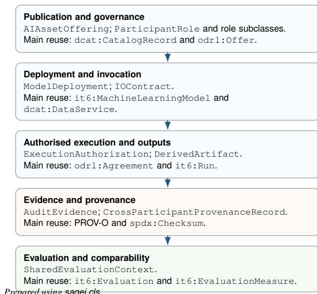
Figure 2. Global functional view of DAIMO by conceptual groupings.
