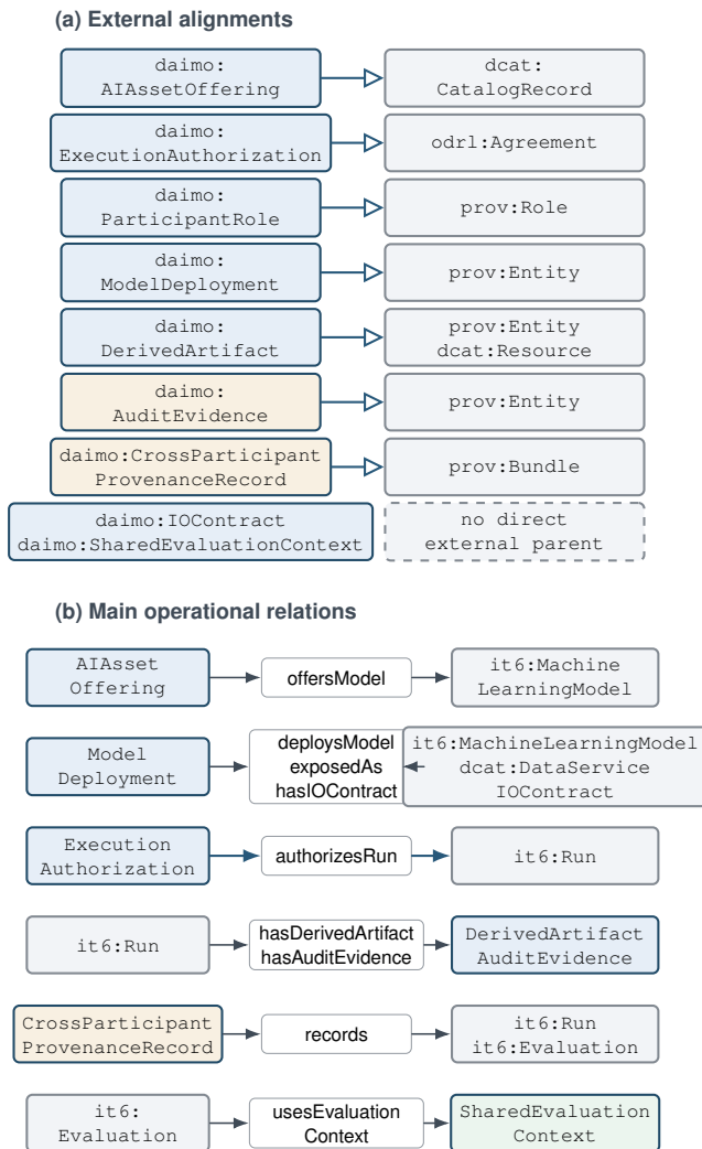
Figure 3. External alignments and main DAIMO relations.
