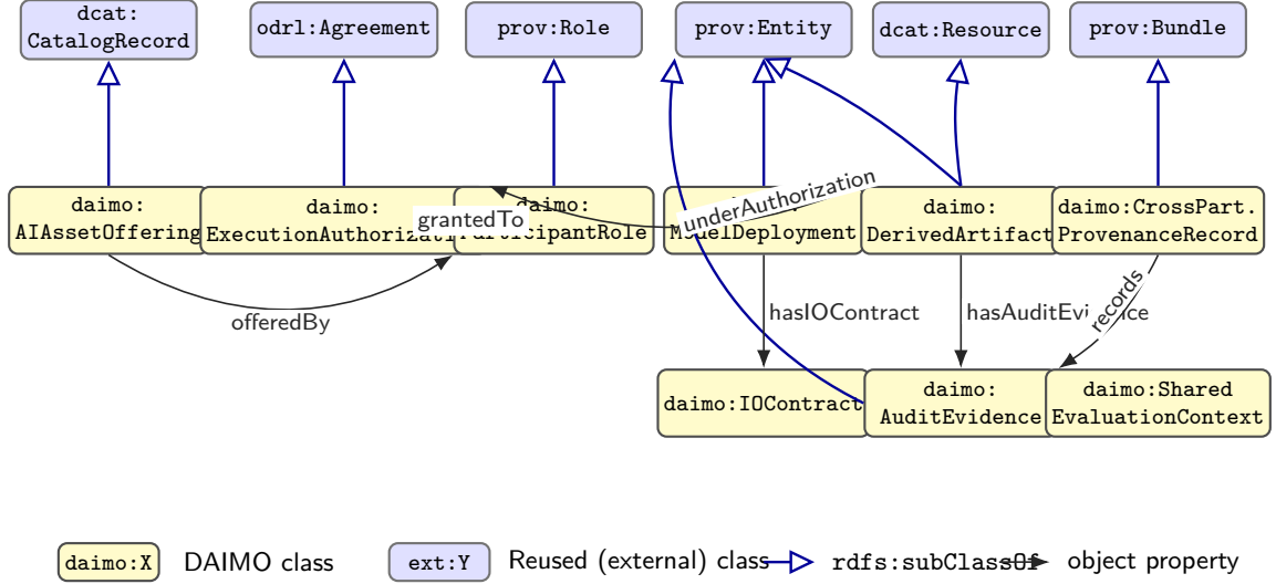
Figure 2: Overview of the DAIMO classes (yellow) with their axiomatic alignments to the reused vocabularies (blue) via rdfs:subClassOf (open-triangle arrows), and the main profile properties that articulate the profile (labelled object-property arrows). DerivedArtifact has two external parents, prov:Entity and dcat:Resource ; AuditEvidence is placed in the bottom row but is also a prov:Entity . Classes IOContract and SharedEvaluationContext carry no external alignment by design. Properties whose targets are classes of the reused vocabularies ( offersModel to it6:MachineLearningModel , authorizesRun to it6:Run ) are declared in Table 6 and are omitted here for readability.
