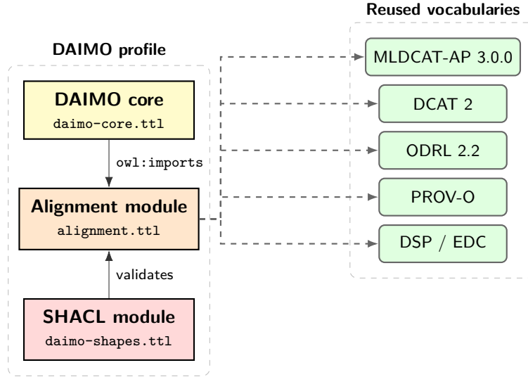
Figure 1: Modular architecture of DAIMO and reused vocabularies. Yellow, orange, and red boxes denote the three DAIMO modules (core, alignment, shapes); green boxes denote the reused vocabularies. Dashed arrows from the alignment module carry the rdfs:subClassOf and rdfs:subPropertyOf declarations. The core module imports alignments for inference; the SHACL module validates data against the combined TBox.
