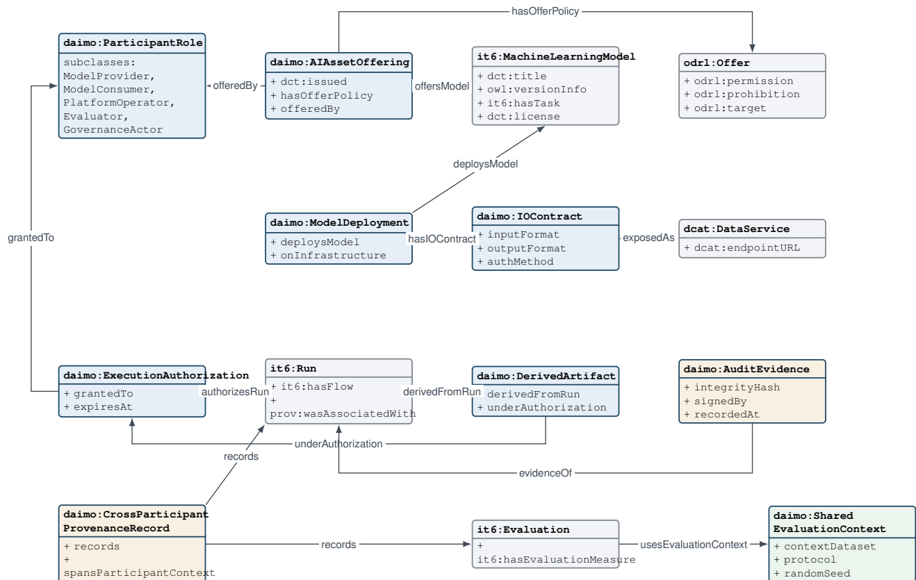
Figure 2. Global ontological view of DAIMO: core bridge classes (blue), reused external classes (grey), evidence classes (amber), and the shared evaluation context (green), with their main attributes and object properties.
