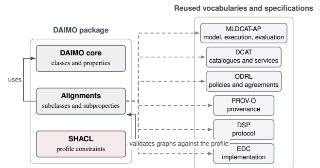
Figure 1. Modular organisation of the DAIMO package and reused resources.
