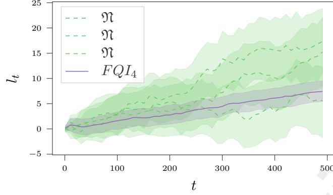
Figure 3.: Average dollar reward l_t of the FQI_4 agent (solid purple line) and those of three identical Normal agents \mathfrak{N} (dashed green lines), when dealing in the same market simulation.
