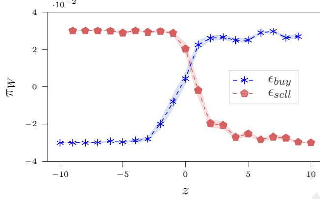
Figure 2.: Equilibrium policy \pi_W for the FQI_2 agents.
