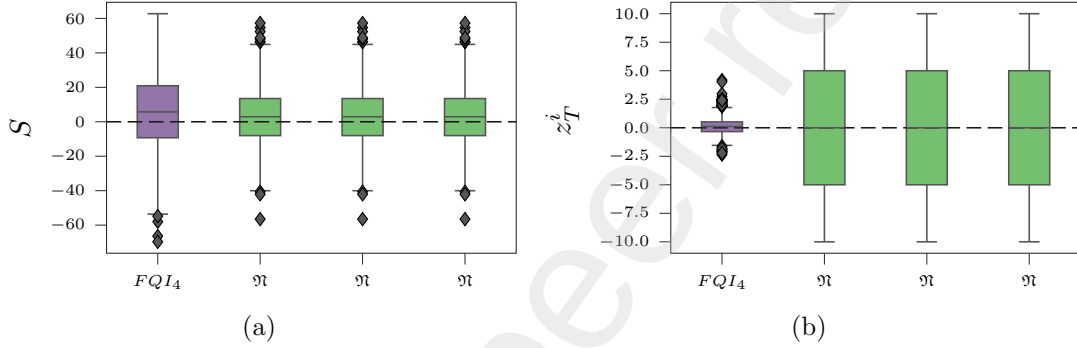
Figure 4.: Box-plot of the distribution over 1,000 runs for (a) Sharpe ratio S ; (b) final inventory z_T^i .
