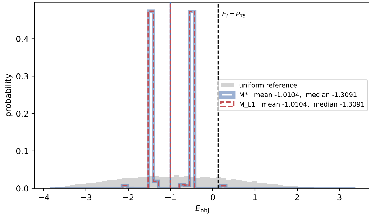
all returned states ( n = 12, p = 3, \text{vseed } 42 )
