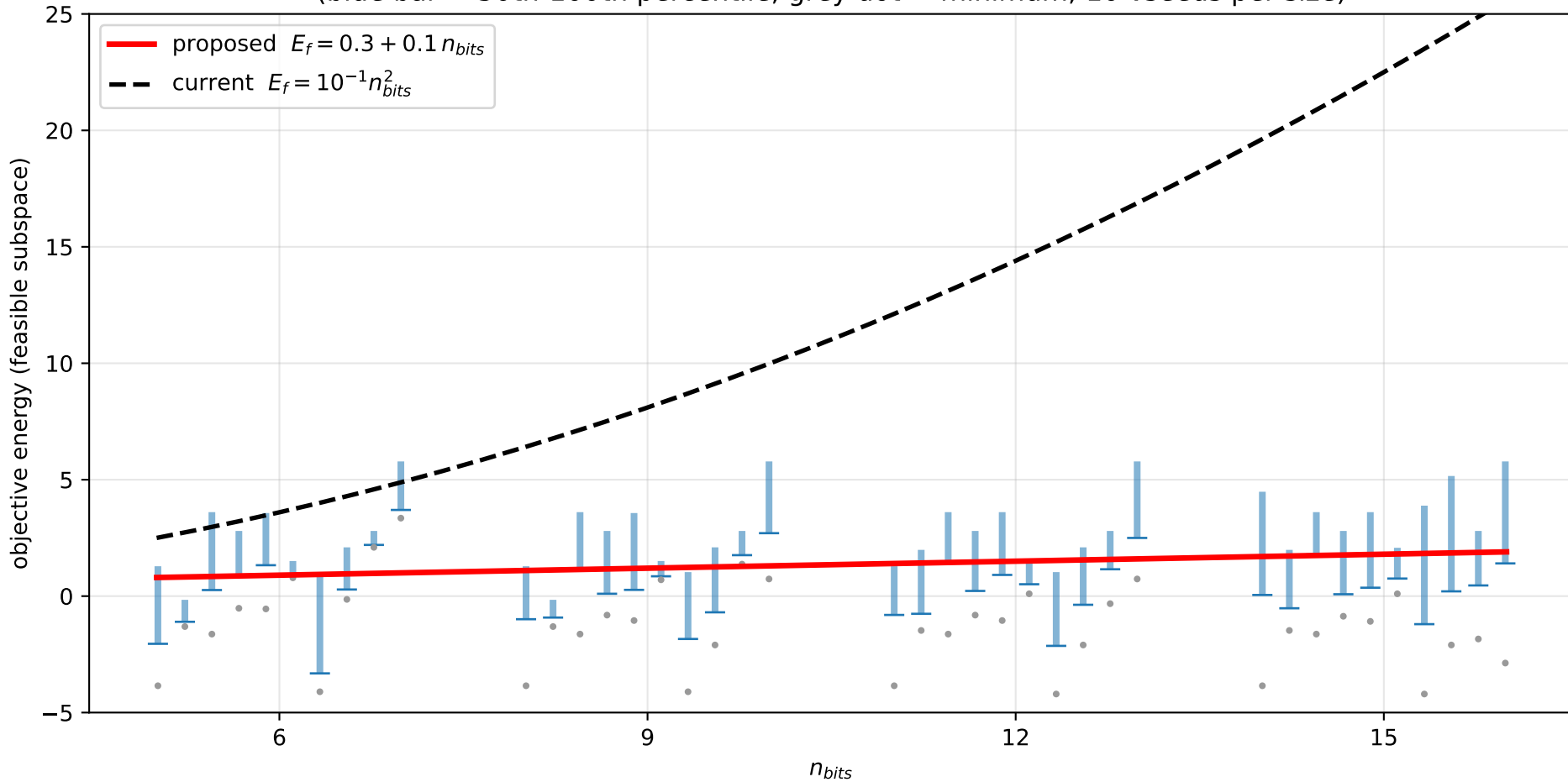
PO: per-instance admissible band [P50, P100] of the feasible objective spectrum (blue bar = 50th-100th percentile, grey dot = minimum; 10 vseeds per size)
