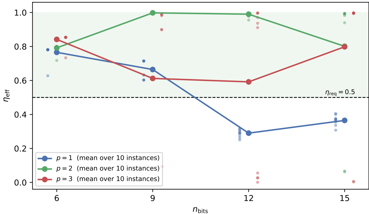
ma-QAOA, PO / optimality, E_f = P_{75} of the feasible spectrum
