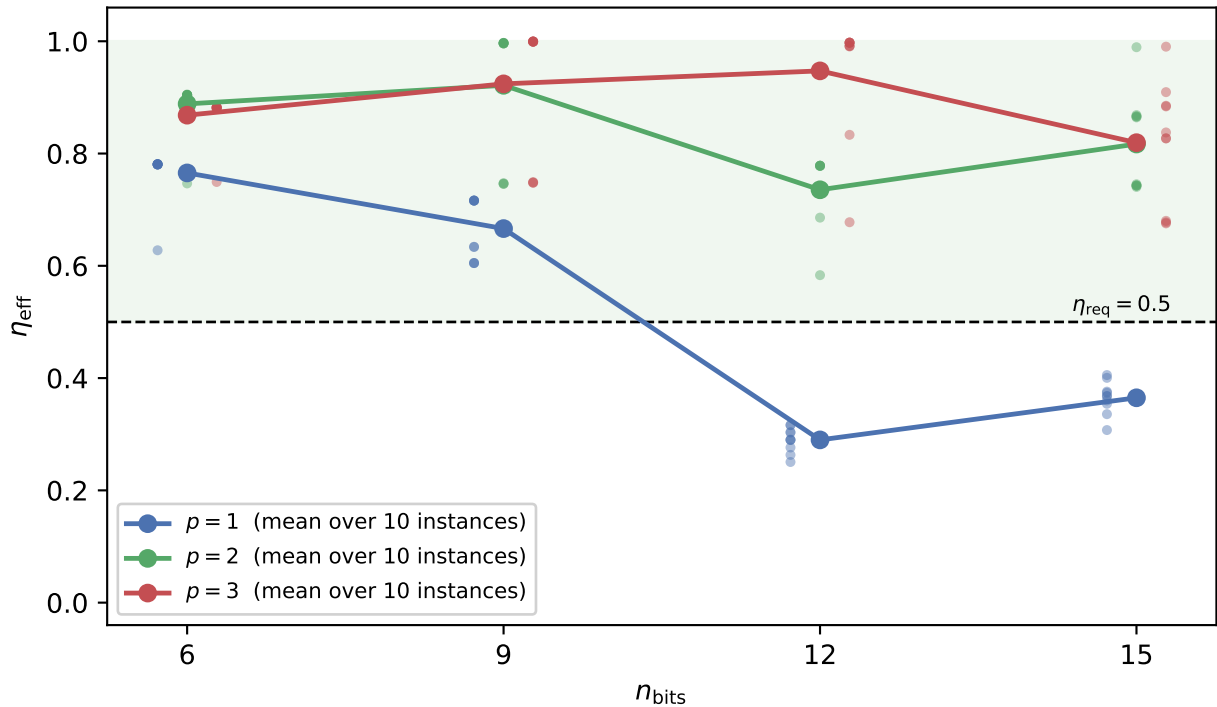
ma-QAOA, PO / optimality, E_f = P_{75} , INTERP warm start
