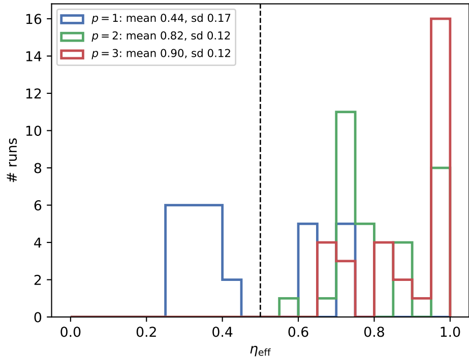
distribution, n_{\text{bits}} \geq 9 (30 runs/depth)
