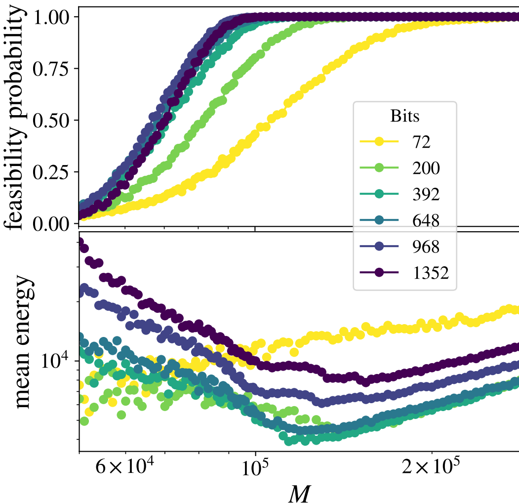
MNPP
