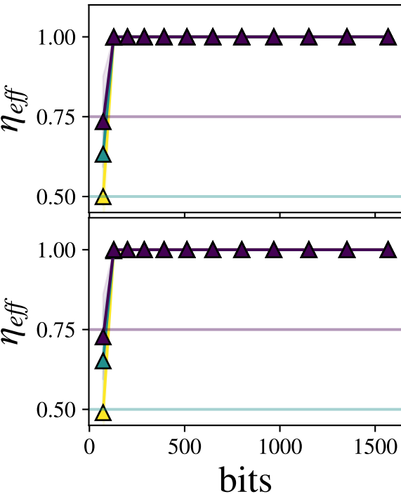
MNPP
