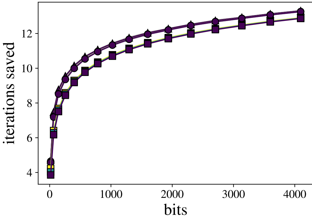
random TSP
