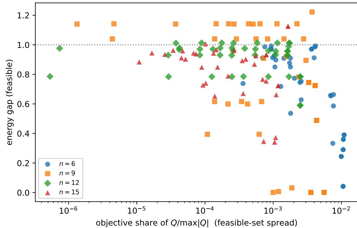
gap vs available signal (corr on \log_{10} share: -0.444, N=161)
