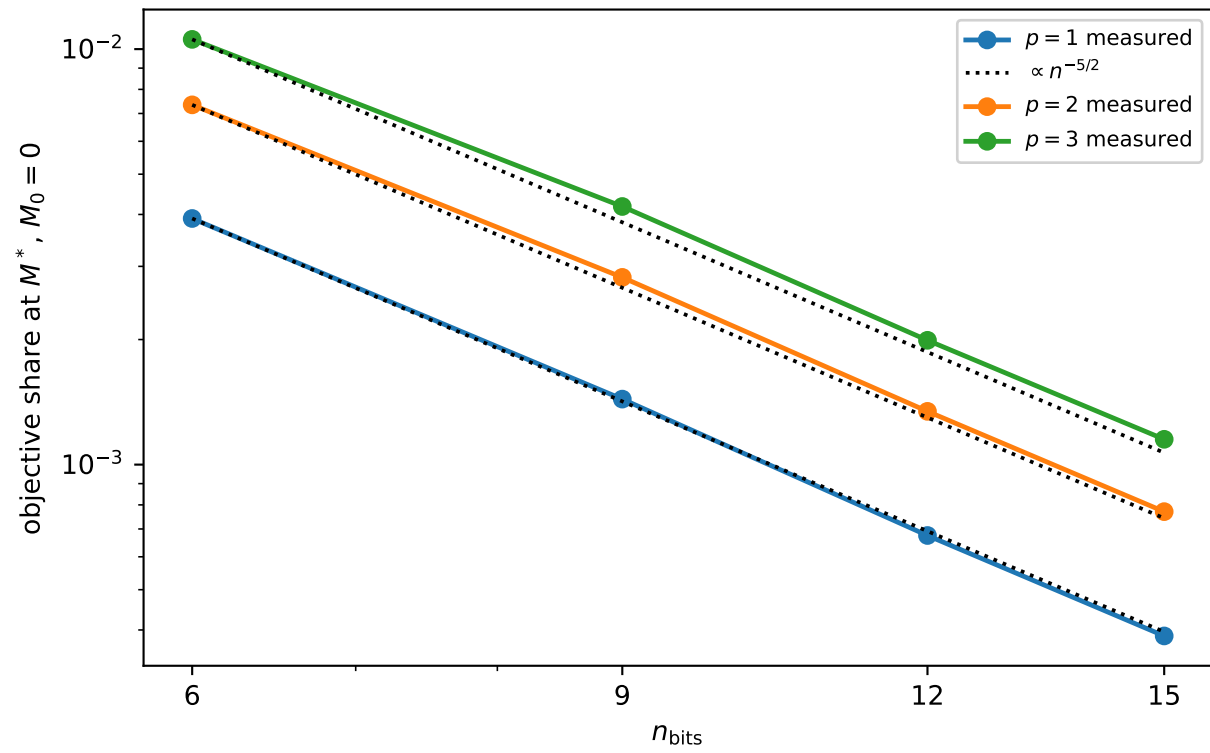
share \sim p/n^{5/2}
