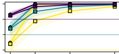
random TSP
