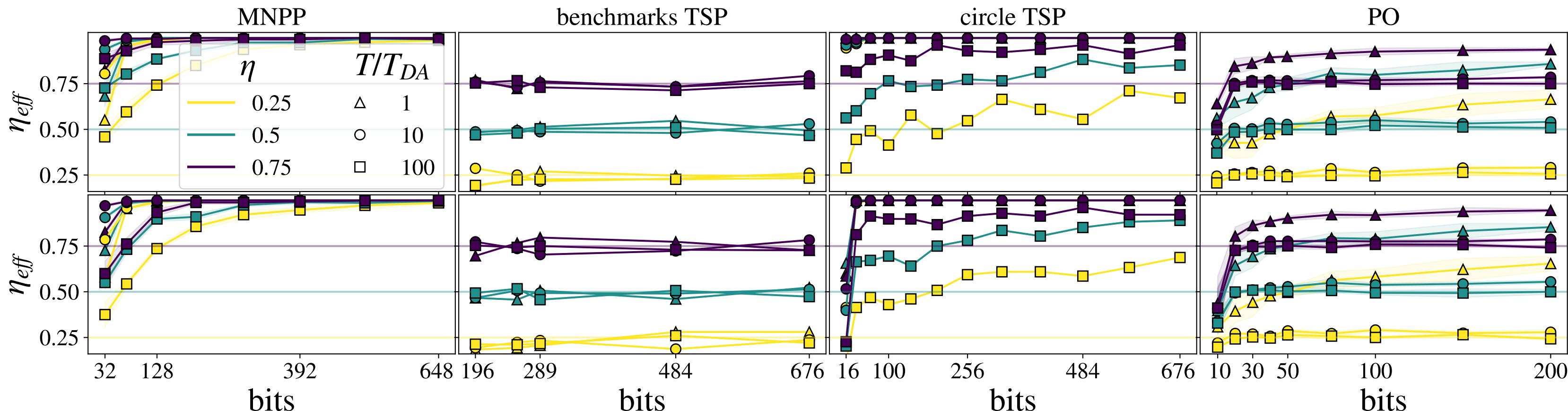
Simulated Annealer
