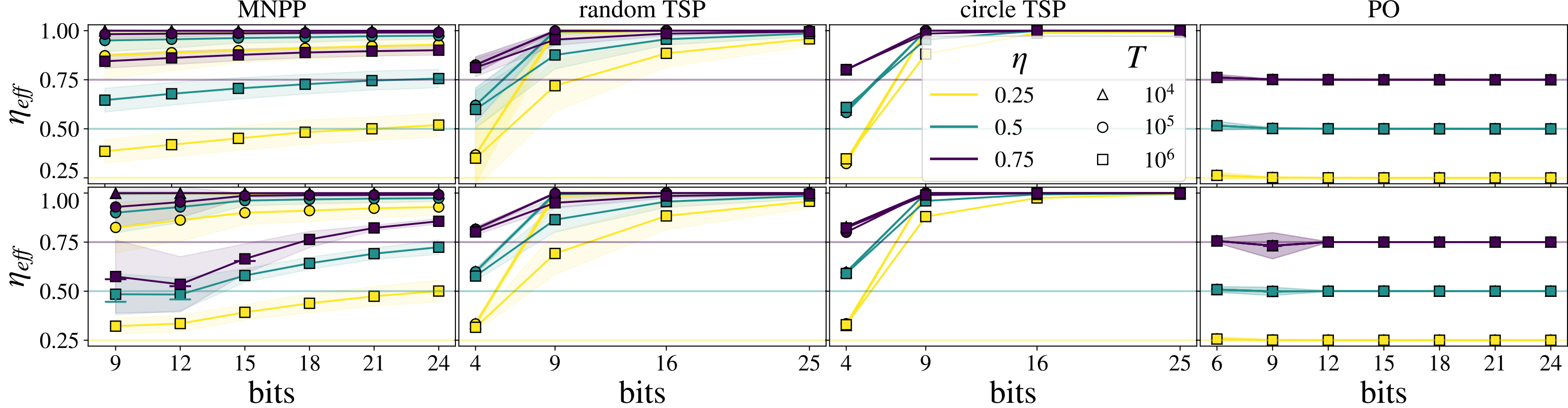
ideal Gibbs sampler
