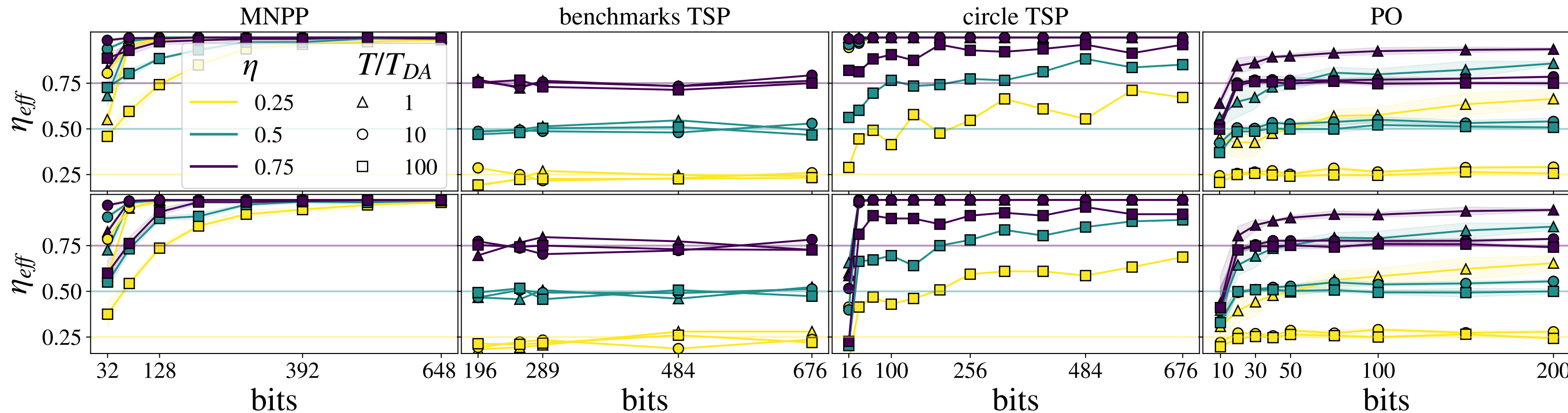
Simulated Annealer
