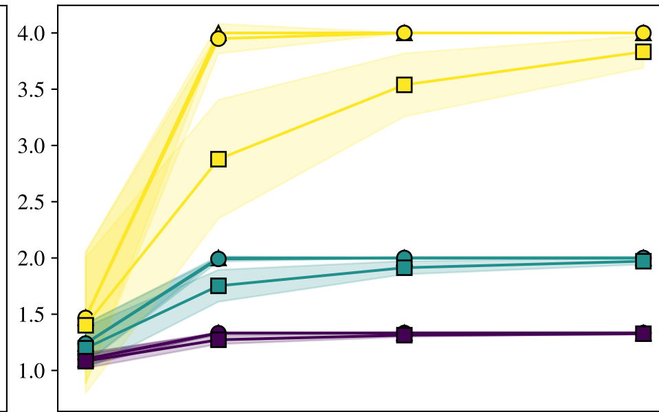
random TSP
