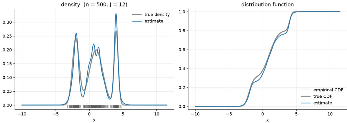
Figure 1: The delivered output on five hundred points from the reference trimodal mixture. Tick marks along the axis are the observations. On the right, the empirical distribution function is drawn underneath and is almost indistinguishable from the other two at this scale.
