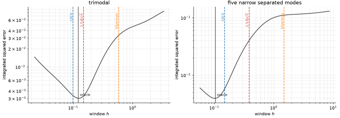
Figure 2: Density error against window width, on two targets, with the choices made by three selectors marked. Both axes are logarithmic. The vertical black line is the best window achievable on that sample.
