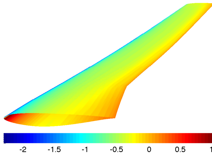
Figure 21. CRM Sub-Scale Model Surface Pressure Map at \alpha = 7.616^\circ and M_\infty = 0.1162
