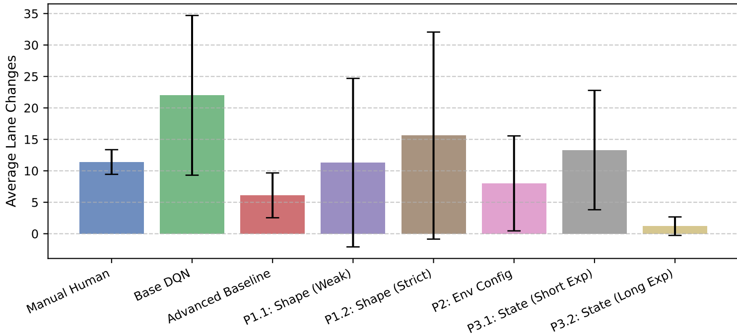
Agent Stability: Lane Changes (P13)
