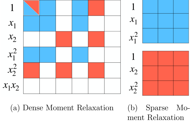
Figure 5.3: Comparison of dense and sparse moment matrices for a two-variable POP at relaxation order \kappa = 2 . Reproduced from [KLY25].
