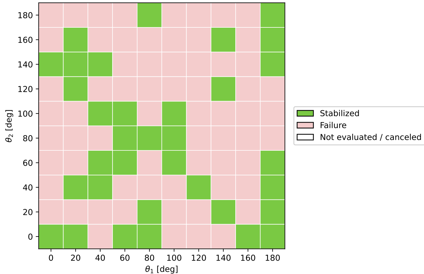
Acrobot basin of attraction ( \Delta t_{SDP} = 0.1 s, \Delta t_{sim} = 0.0025 s)
