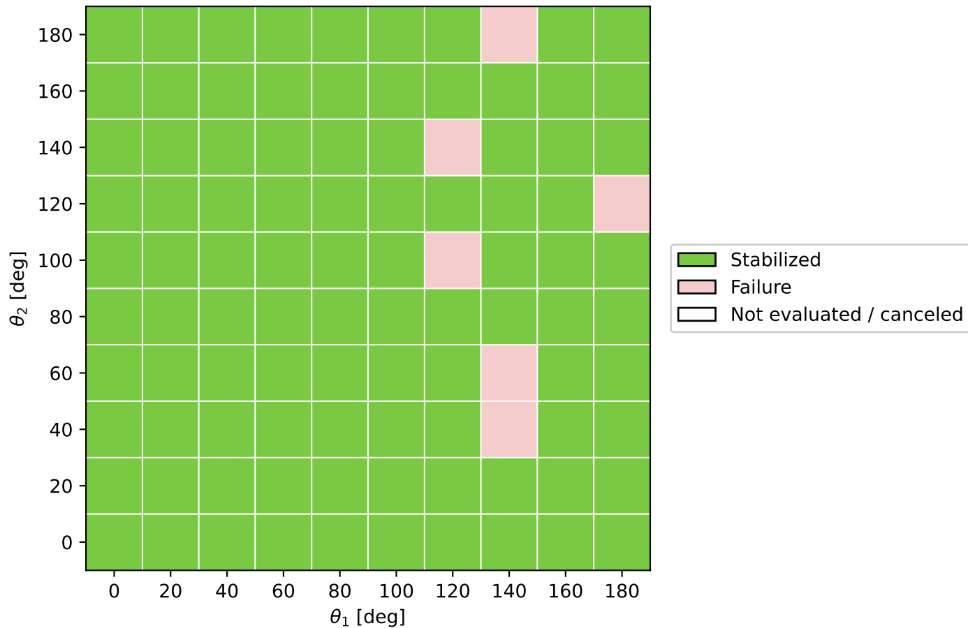
Acrobot basin of attraction ( \Delta t_{SDP} = 0.1 s, \Delta t_{sim} = 0.1 s)
