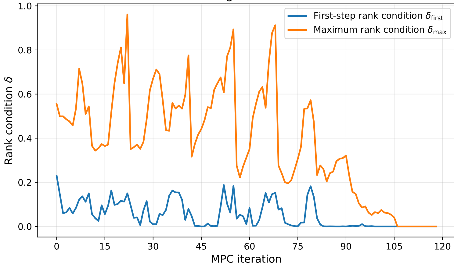
Moment-relaxation tightness over MPC iterations
